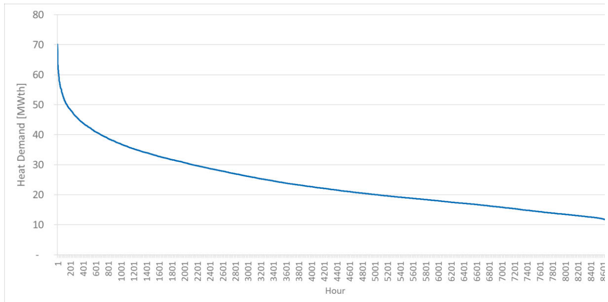
Figure 5: Heat load duration curve
