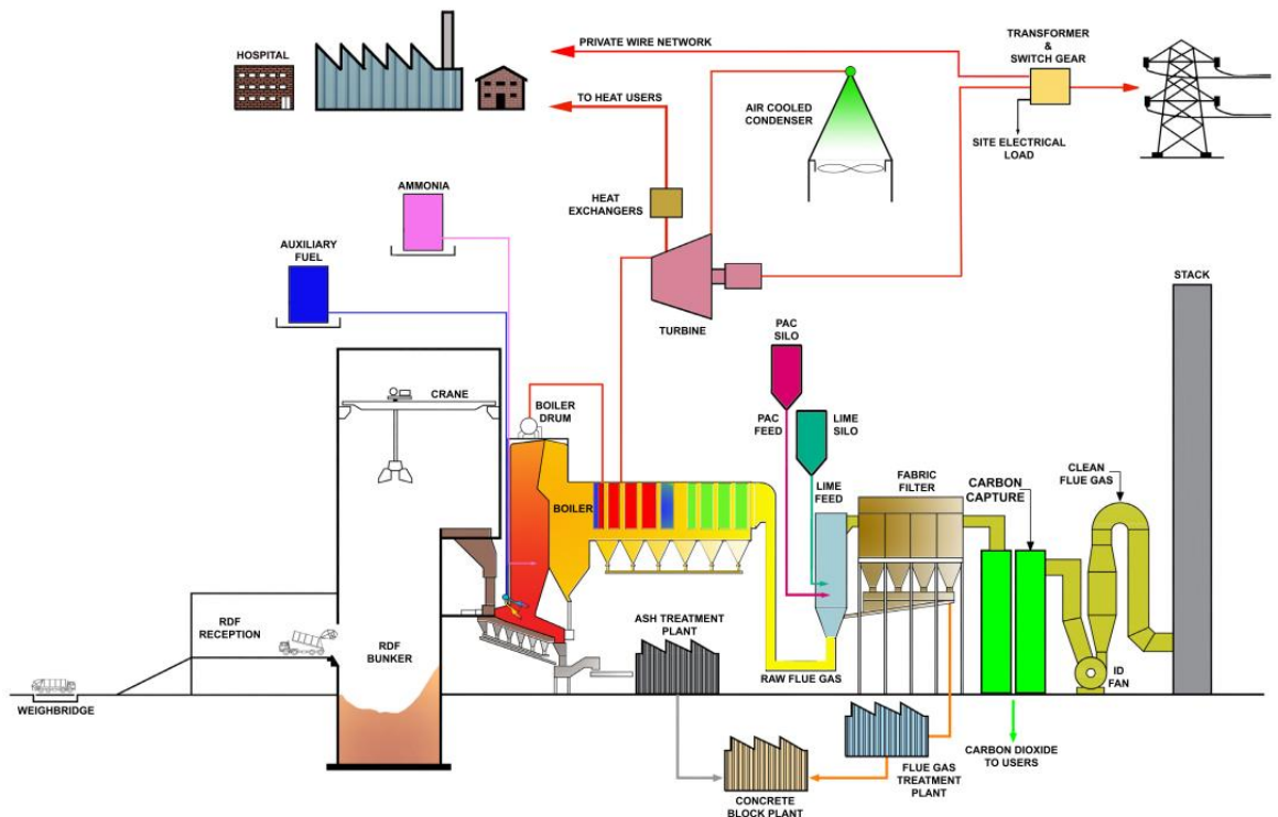
Figure 2: Process schematic
